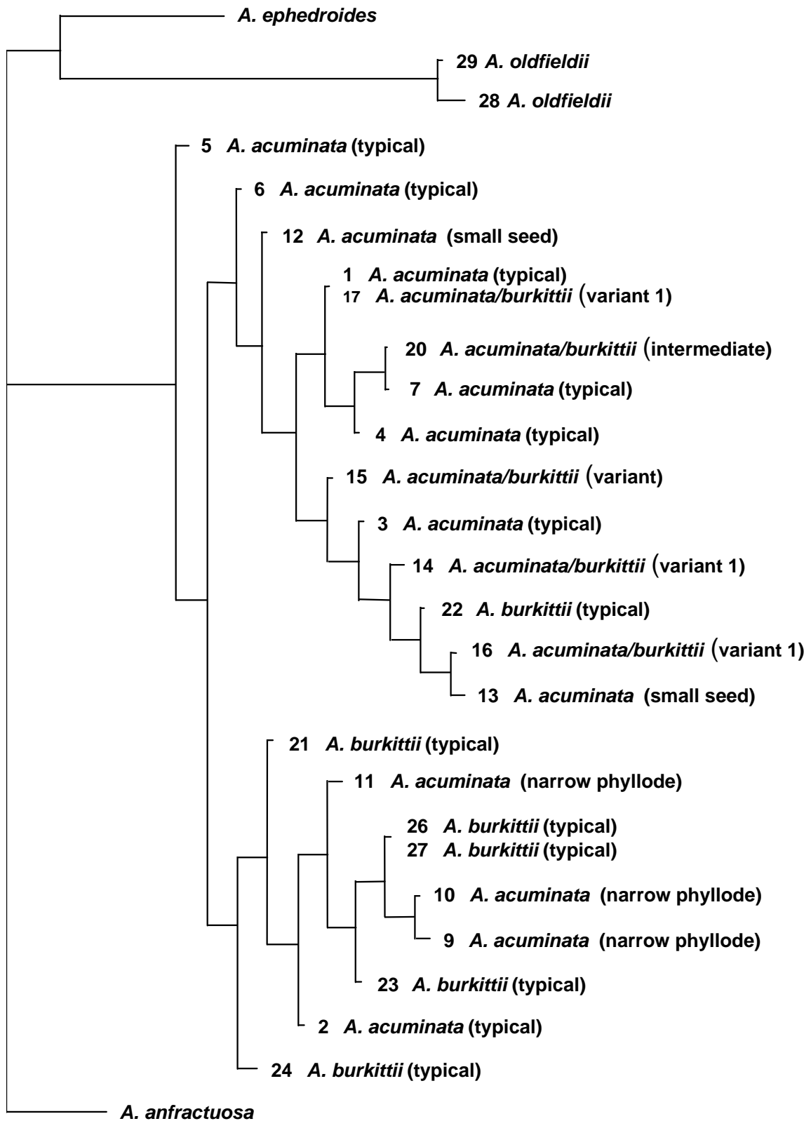
Figure 6. Relationships between populations of the A. acuminata complex based on chloroplast DNA analysis. The numbers on the end of branches are population numbers.
